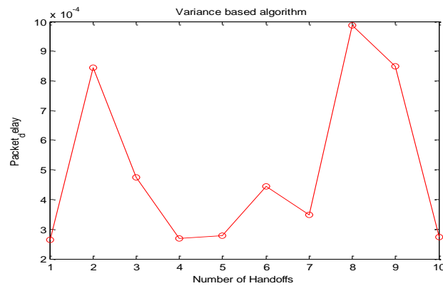
Fig 5.4 Packet delay vs number of handoffs for variance based algorithms
