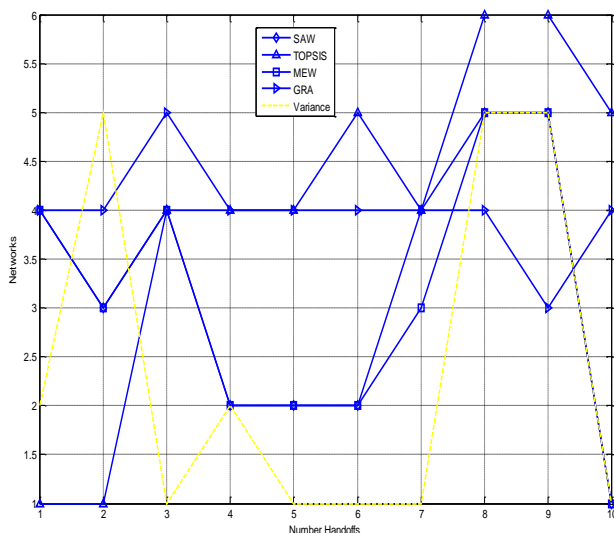
Fig 5.1 Network selection by the various algorithms
