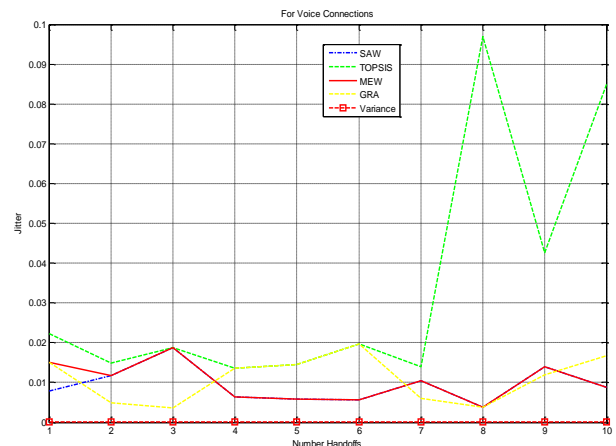
Fig 5.3 Jitter vs number of handoffs for various algorithms
