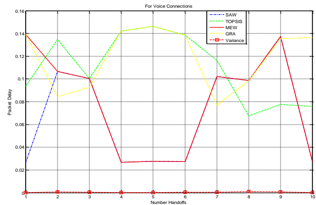
Fig 5.2 Packet delay vs number of handoffs for various algorithms
